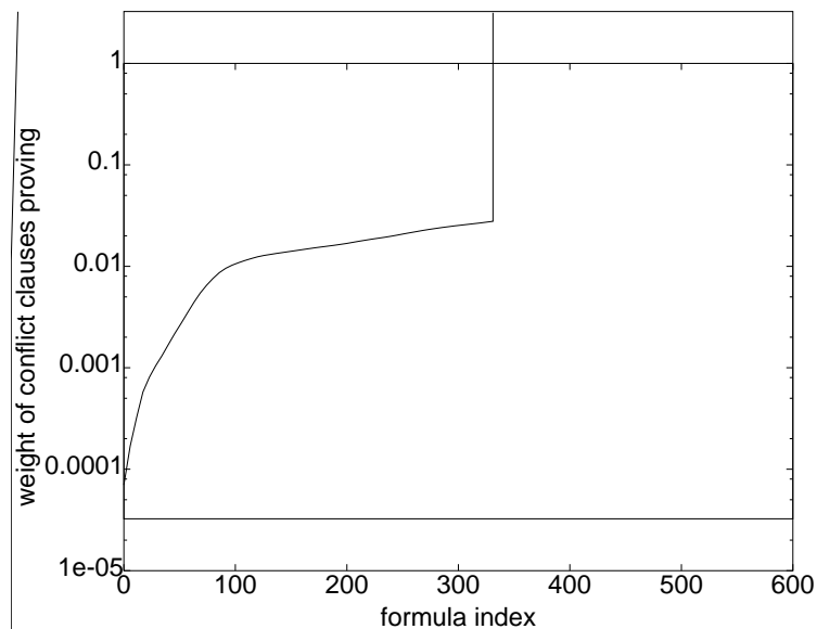
Figure 4: weight of the conflict clauses proof generation
